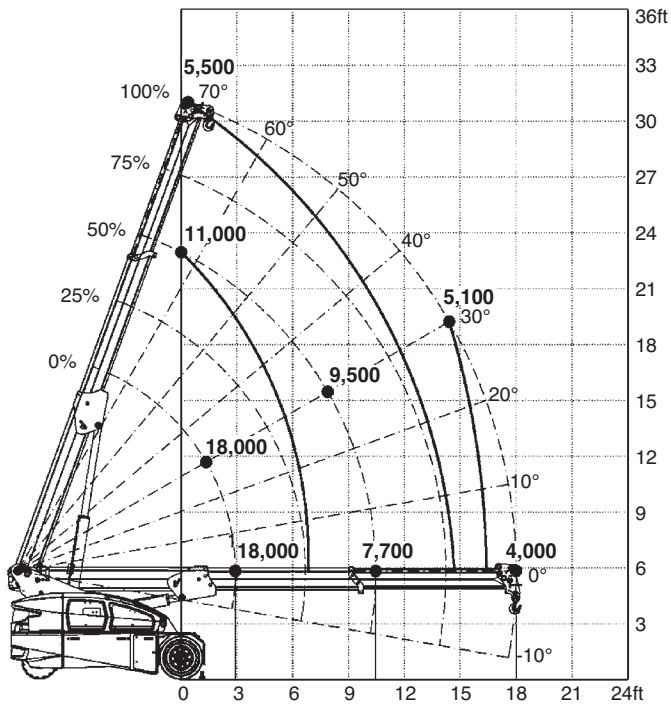
Main Boom – Stabilizer Lifted Pick & Carry Hook
