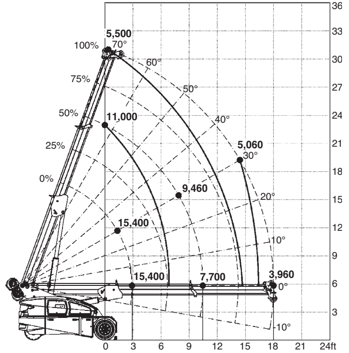
Main Boom & Hydraulic Jib – Stabilizer Deployed Winch & Wire Rope
